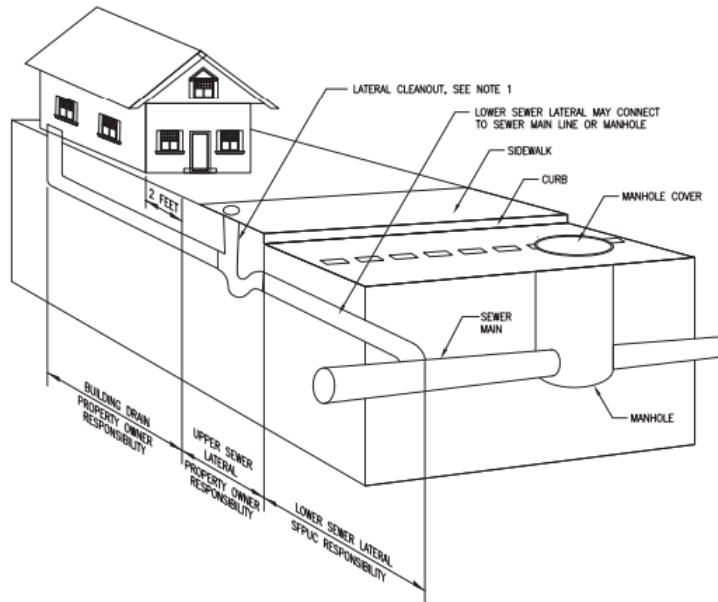
FIGURE 20: COMPONENTS OF THE COMBINED SEWER SYSTEM
