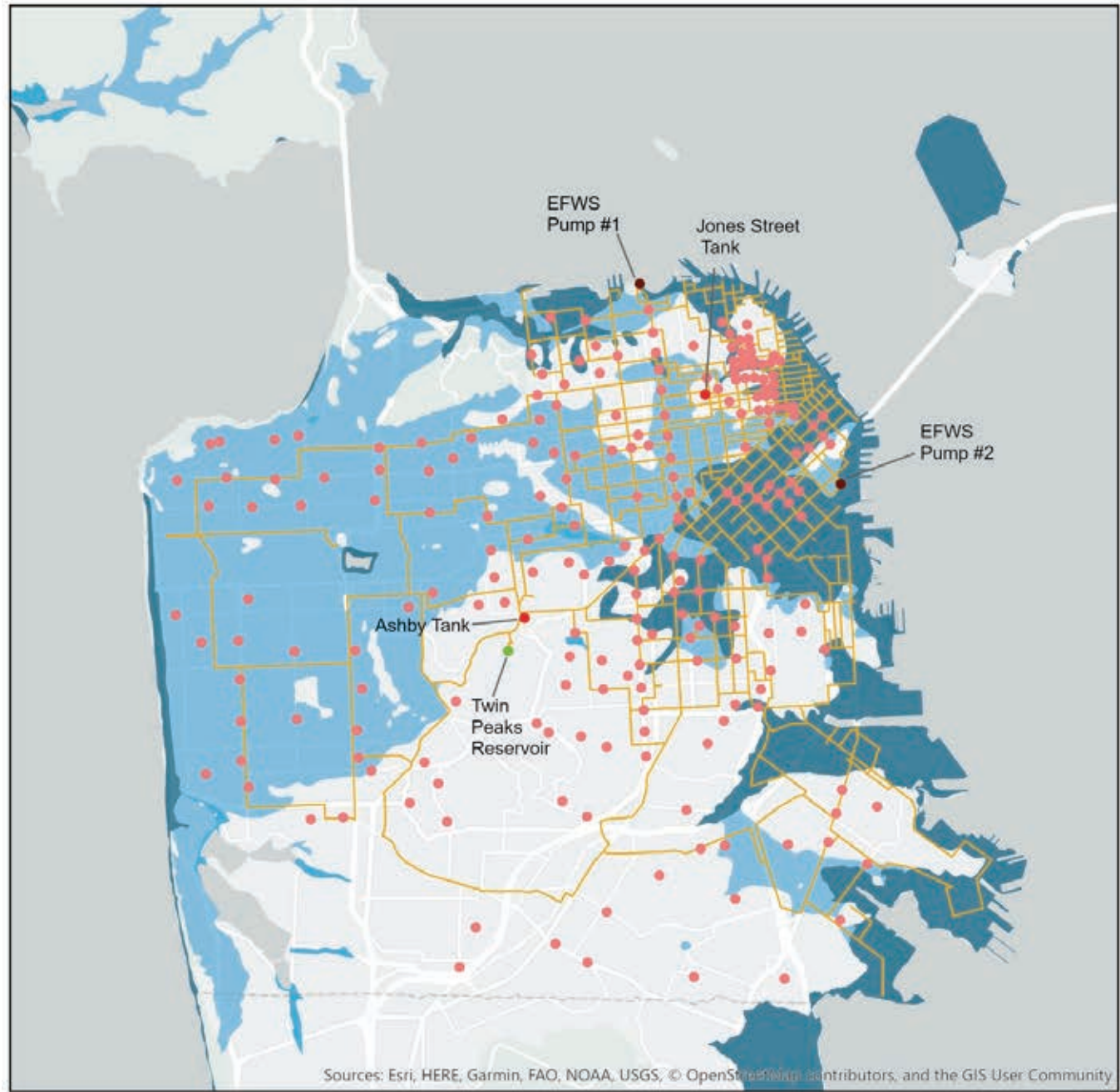
FIGURE 29: EFWS SYSTEM MAP
