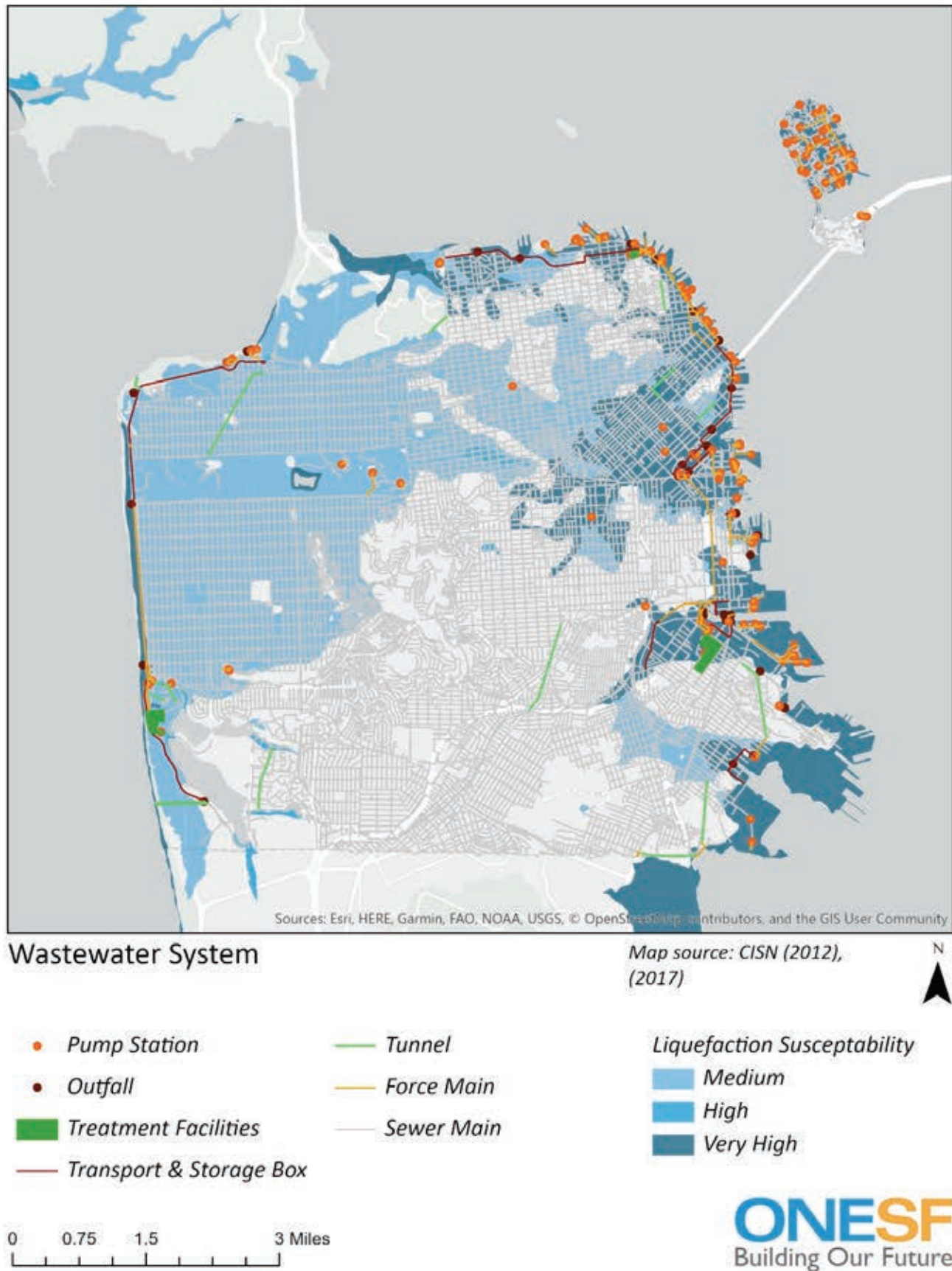
FIGURE 21: WASTEWATER SYSTEM MAP
