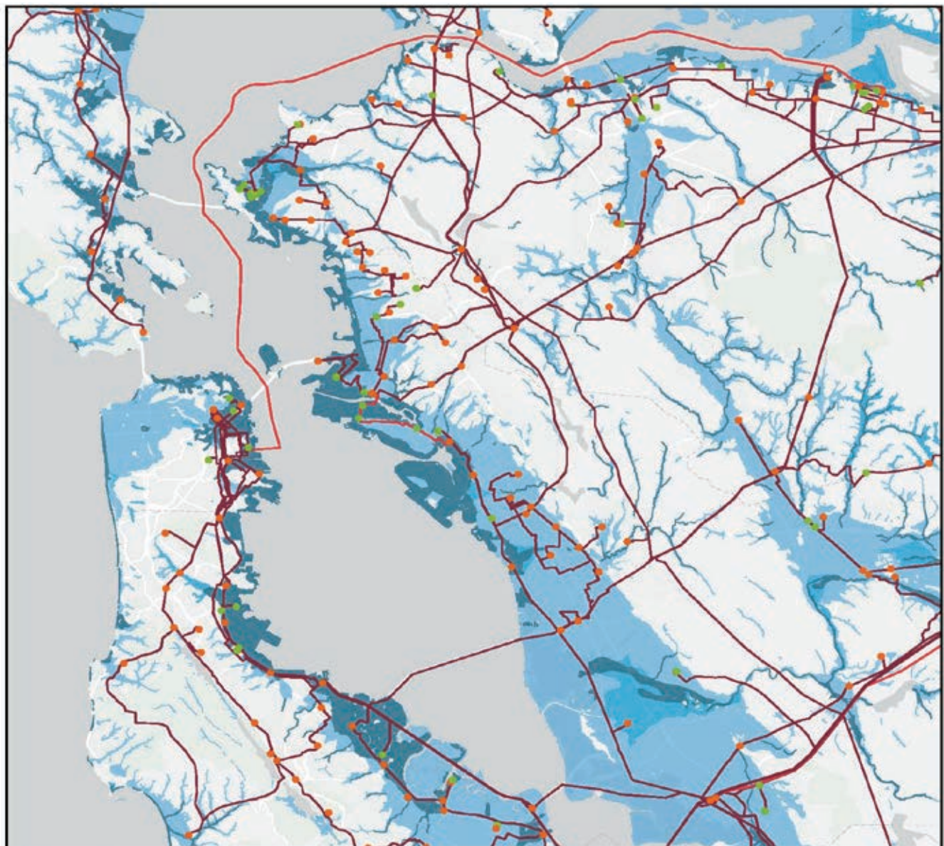
FIGURE 7: ELECTRIC POWER SYSTEM MAP
